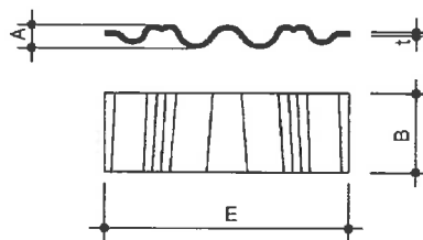
Wellennagel Form 2
